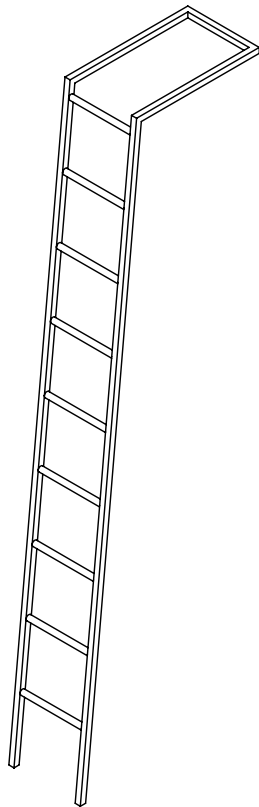
LADDER ISOMETRIC VIEW
