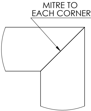
DETAIL X SCALE 1 : 1
