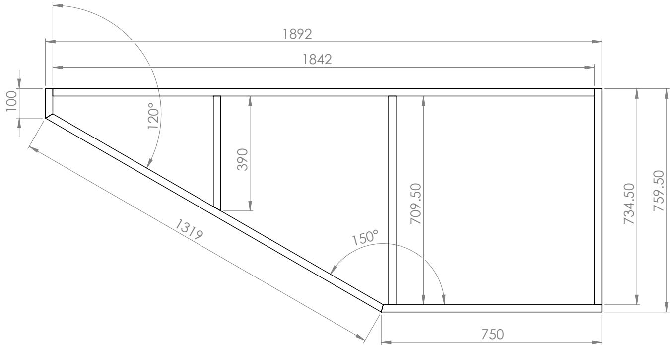
PLYNTH A. TOP VIEW
