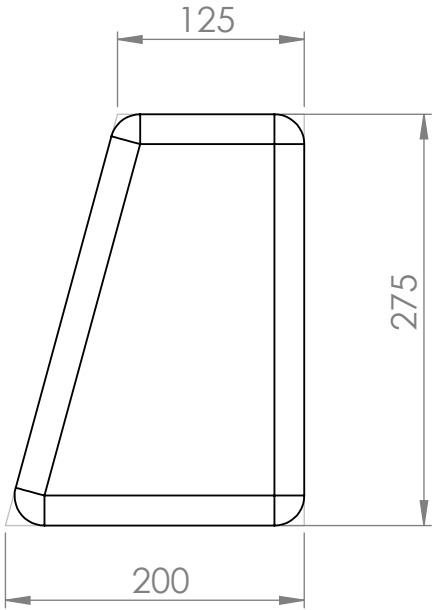
BACK CUSHION - MAIN SIDE VIEW
