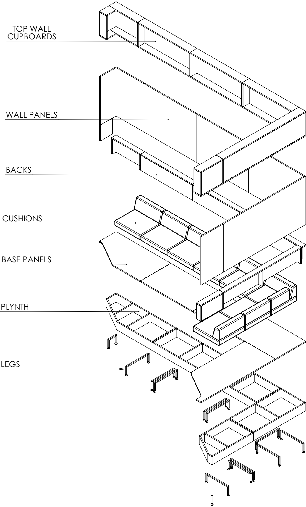
RHS L-SHAPE BOOTH EXPLODED VIEW
