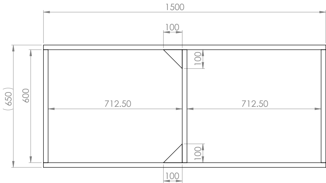
PLYNTH A TOP VIEW
