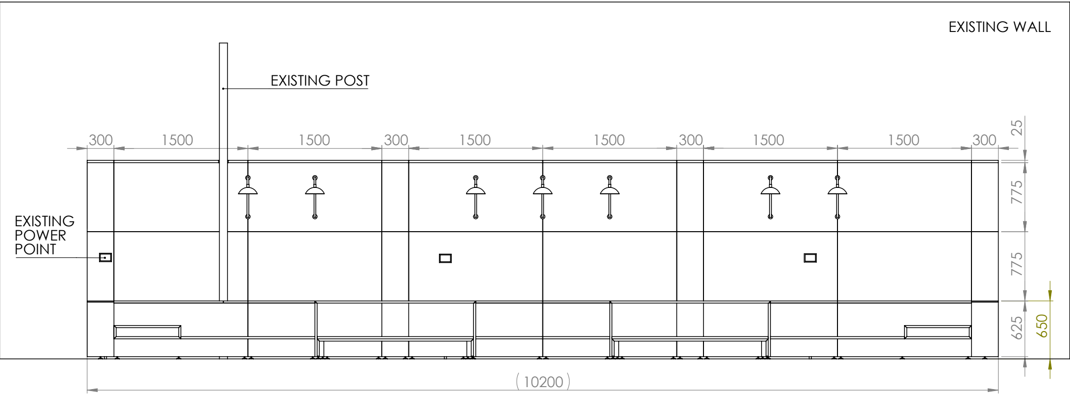
FRONT VIEW - NO CUSHIONS
