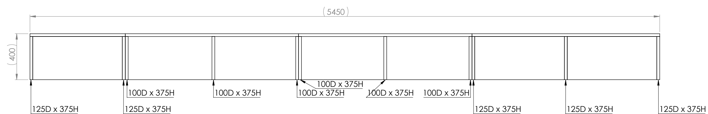
BACK VIEW
