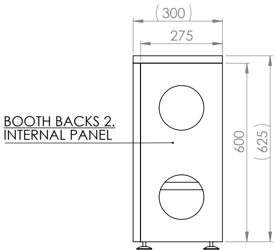
RHS SIDE VIEW
