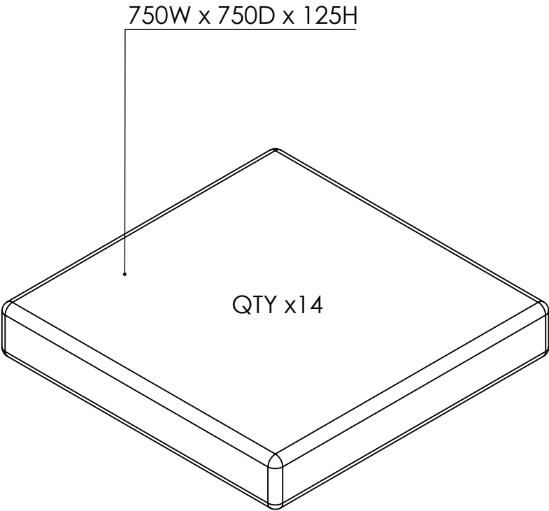
SEAT CUSHION ISOMETRIC VIEW
