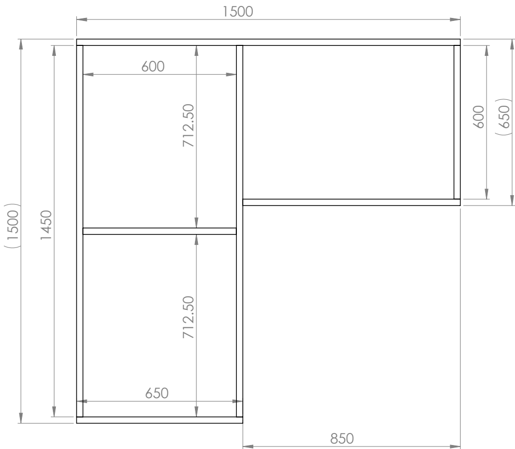
PLYNTH A TOP VIEW
