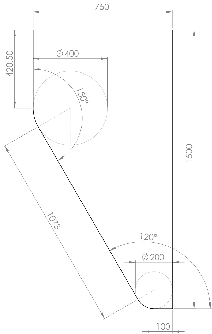
TOP VIEW SIDE TABLE
