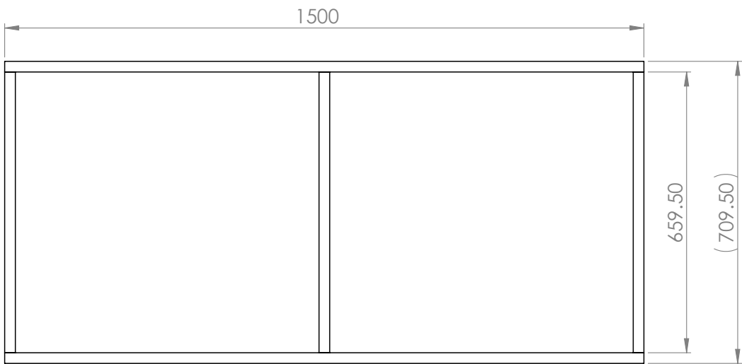
PLYNTH B. TOP VIEW QTY x3
