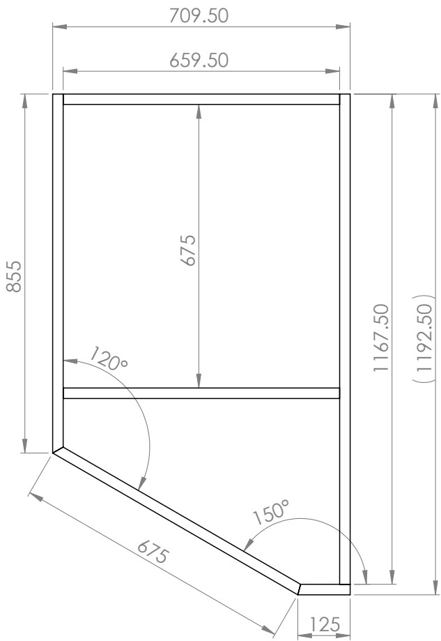
PLYNTH C. TOP VIEW
