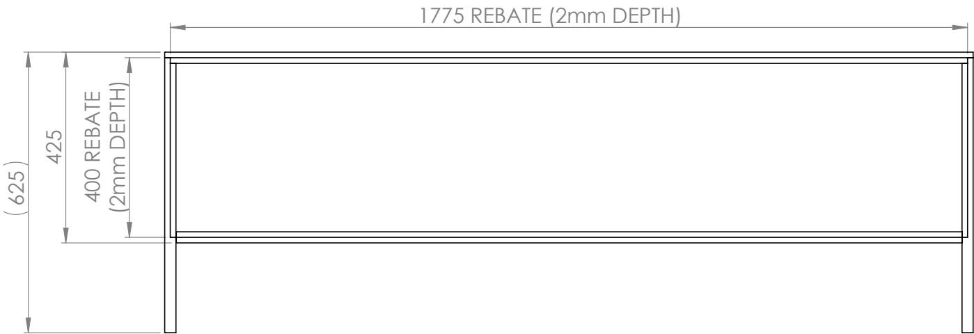
BACK STORAGE 2. BACK IS REBATED THE SAME AS STORAGE 1. (THIS CABINET IS JUST LONGER)
