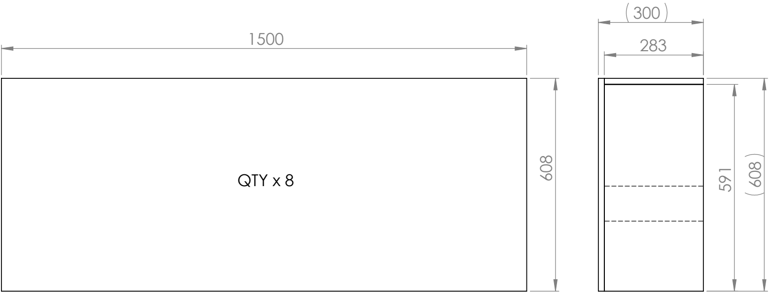
SIDE SECTION VIEW
