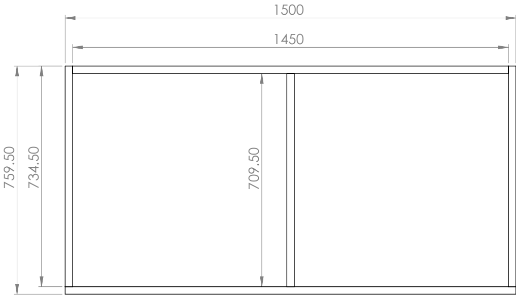
PLYNTH B. TOP VIEW
