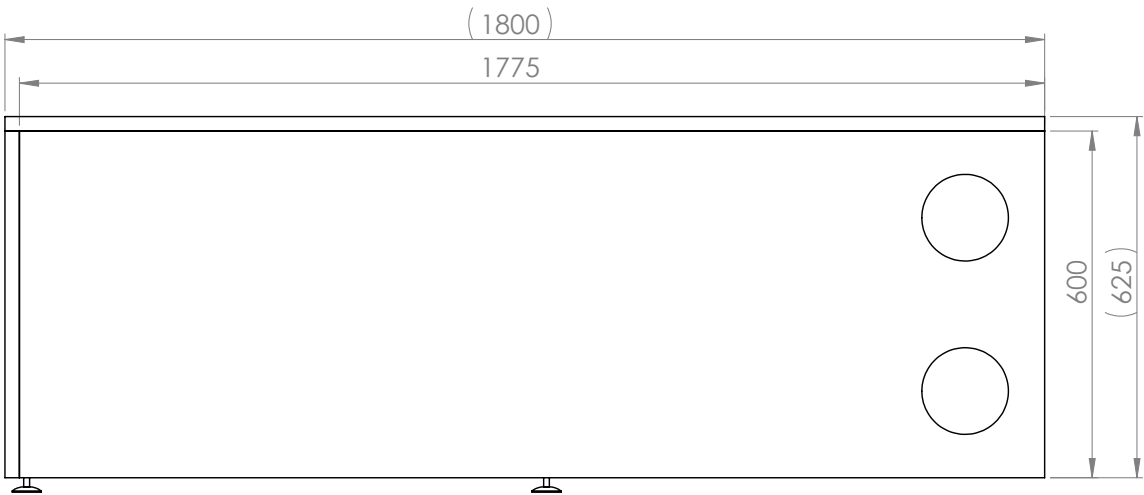
RHS SIDE VIEW
