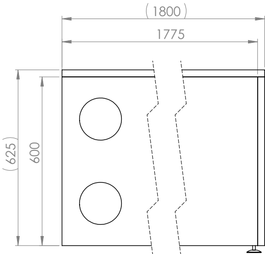
LHS SIDE VIEW
