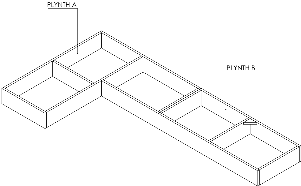
PLYNTH A ISOMETRICVIEW
