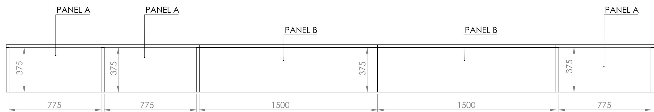
FRONT VIEW
