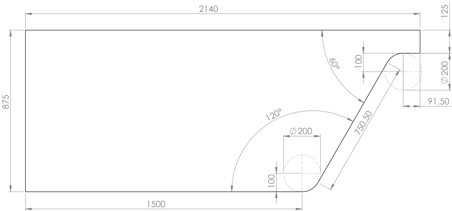
PANEL D TOP VIEW
