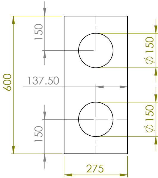
BOOTH BACKS 2. INTERNAL PANEL QTY x16
