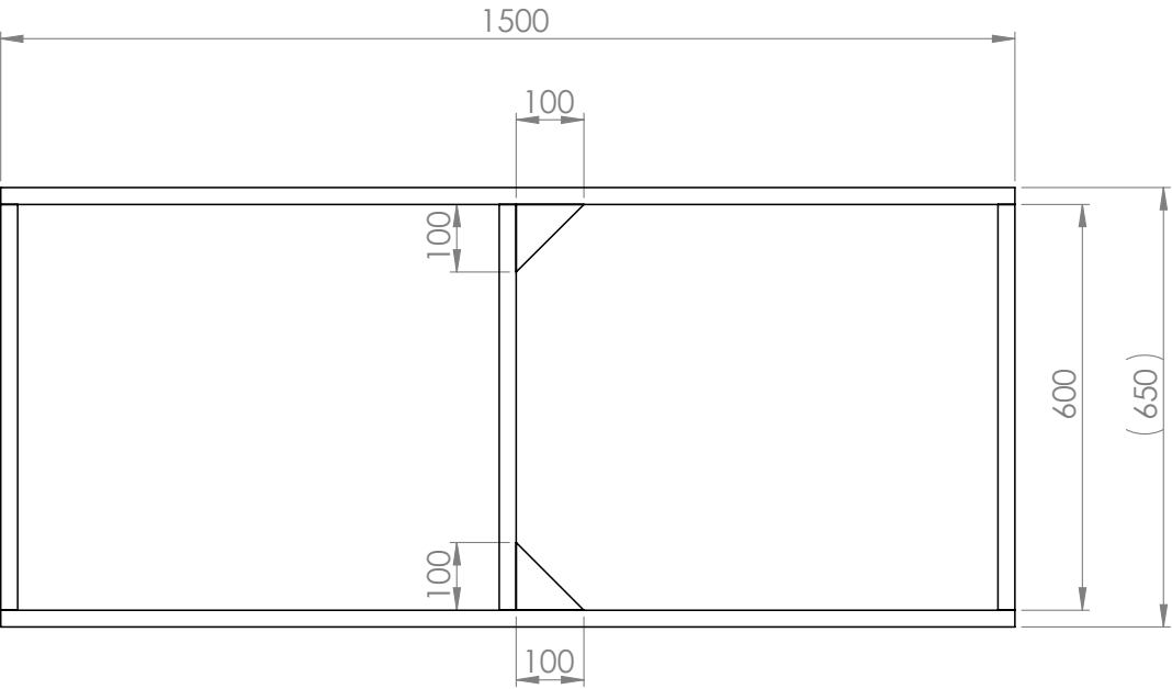
PLYNTH B TOP VIEW
