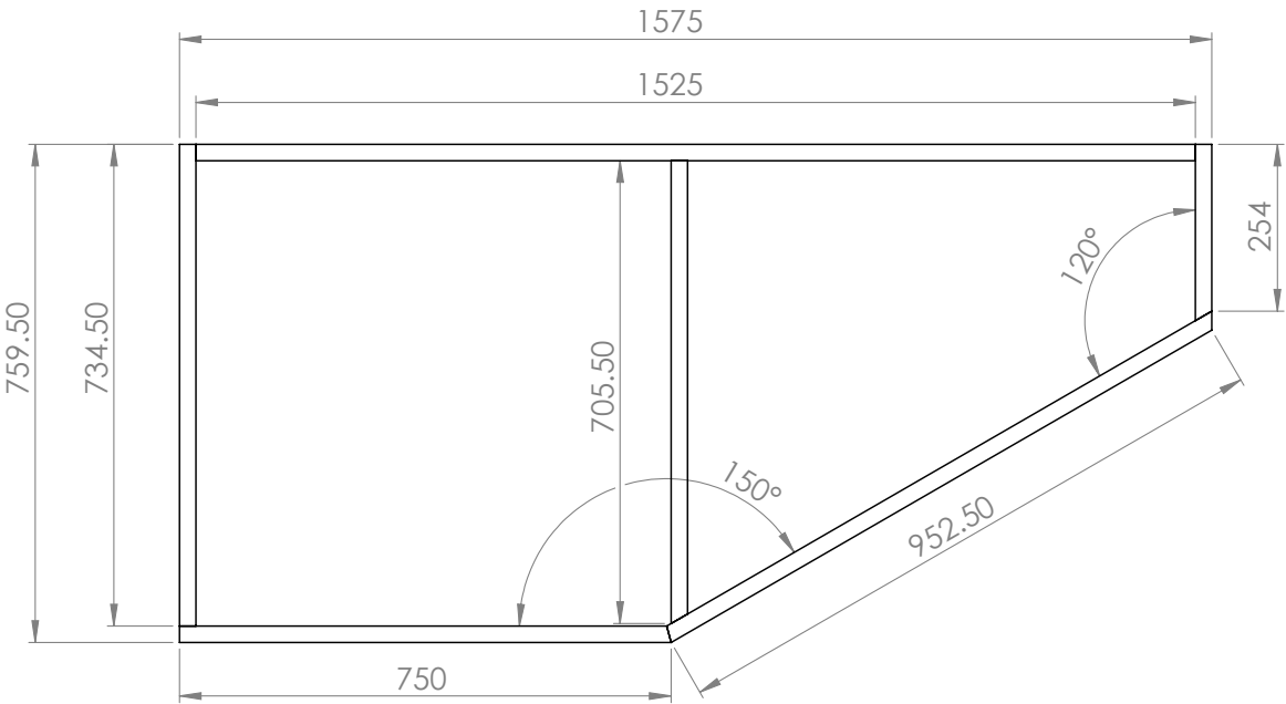
PLYNTH C. TOP VIEW
