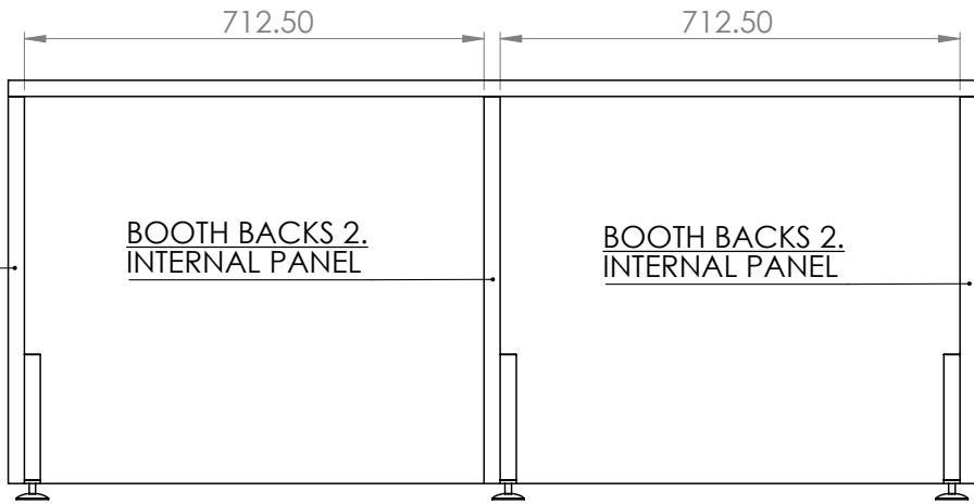
BACK VIEW (NO BACK PANEL - OPEN)
