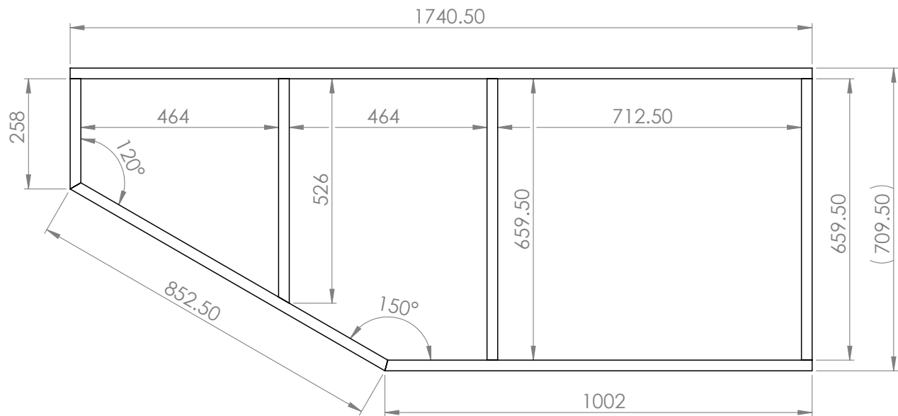
PLYNTH A. TOP VIEW
