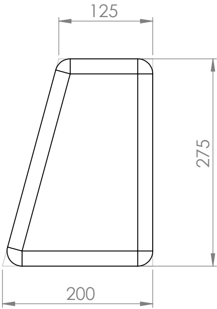
BACK CUSHION - MAIN SIDE VIEW
